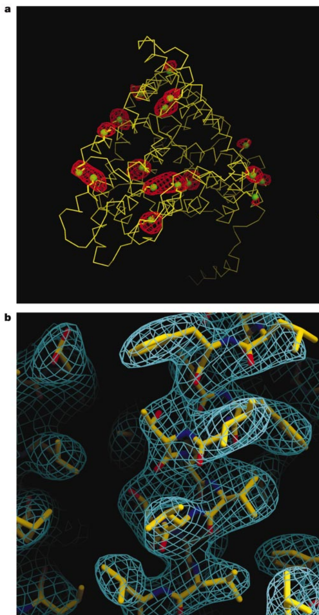
Figure 2 Experimental electron density. a , F_{Se} - F_{native} difference density (contoured at 4\sigma ) in the EcCIC P2_1,2_1 crystal form superimposed on an \alpha carbon trace of the EcCIC subunit viewed from outside the cell. Side chains of methionine residues are shown in stick representation with the position of the Se atom indicated by a green sphere. The difference Fourier map was calculated to 4.0 Å and averaged over the six subunits in the asymmetric unit. b , Electron density map from the StCIC P2_1 crystal form at 3.0 Å resolution, contoured at 1\sigma . The map was calculated from native amplitudes and solvent-flattened, averaged phases. The refined structure is shown as a stick model. Figures 2–6 were prepared with DINO ( http://www.dino3d.org ).
